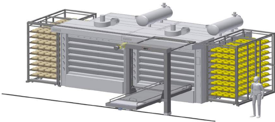
SA - Automatic system with a docking station
