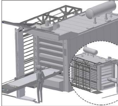
SPA - Semi-automatic system with docking station
